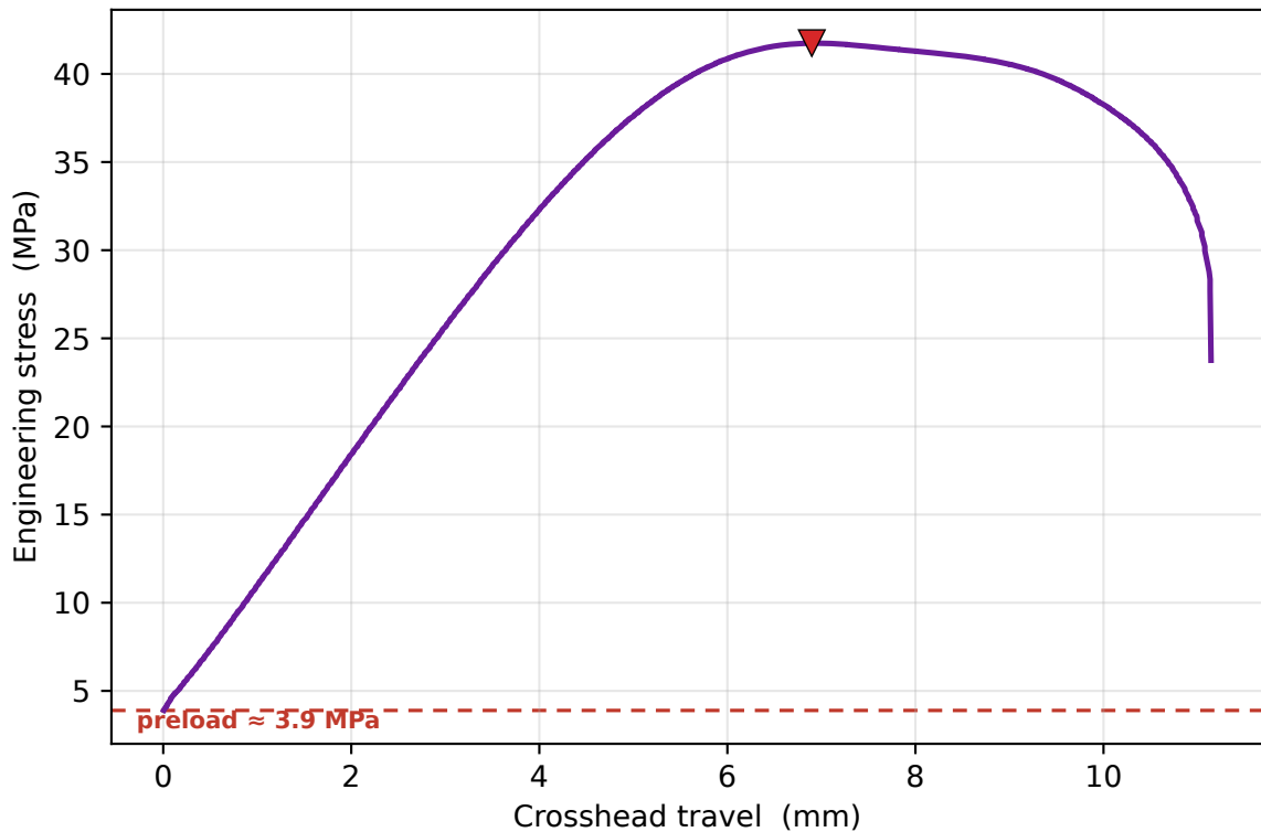
Stress vs crosshead
